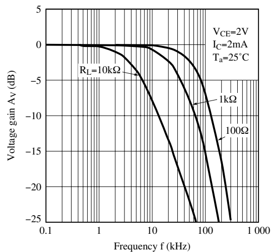
Fig.16 Frequency Response
