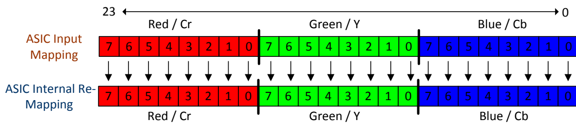
Figure 9. 24-Bit Rgb-888 I/O Mapping
