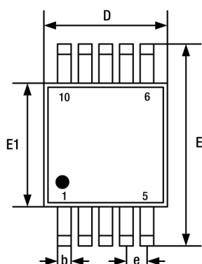
Package top view
