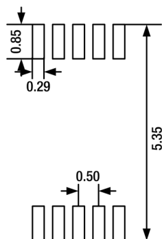
Recommended solder pads
