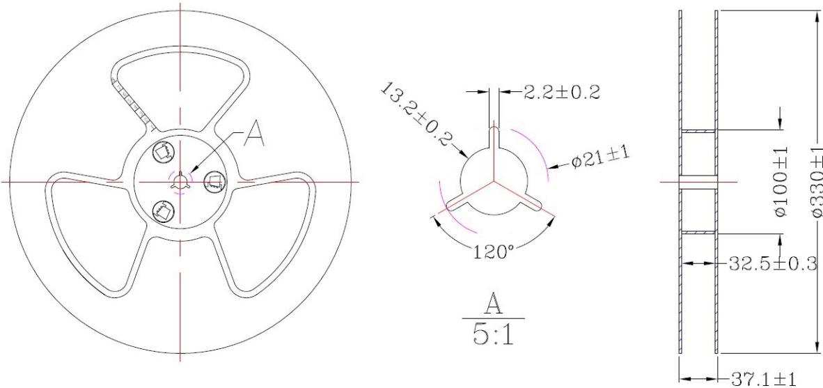
Figure 16: Reel Dimensions
