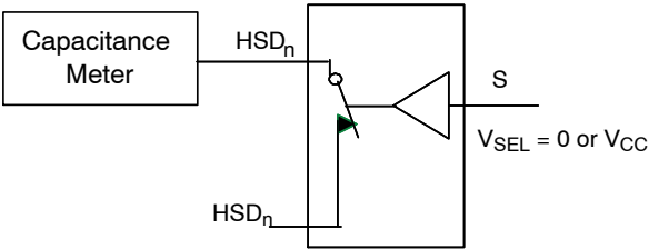
Figure 12. Channel On Capacitance
