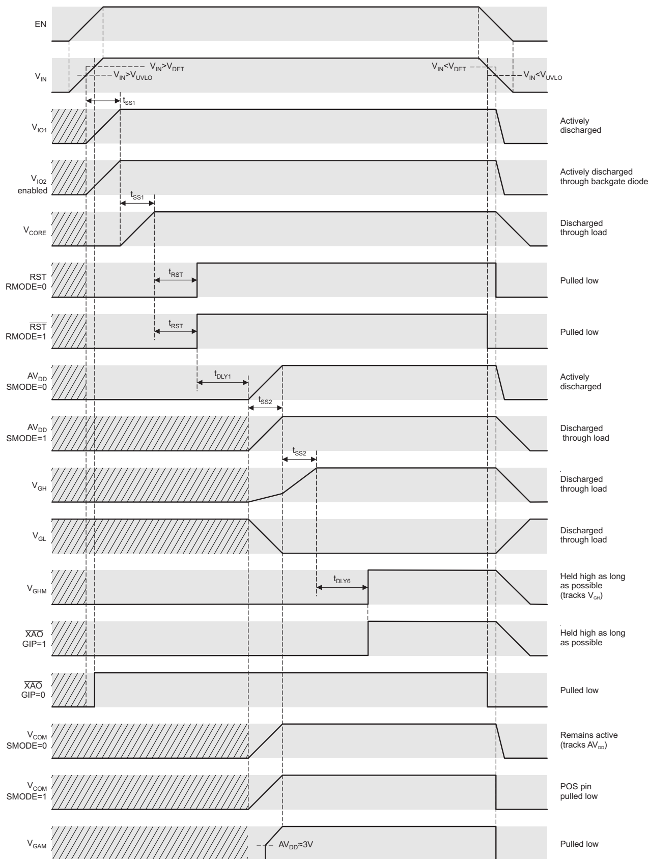
Figure 5-41. Power Up/Down Sequencing with EN Connected to V IN
