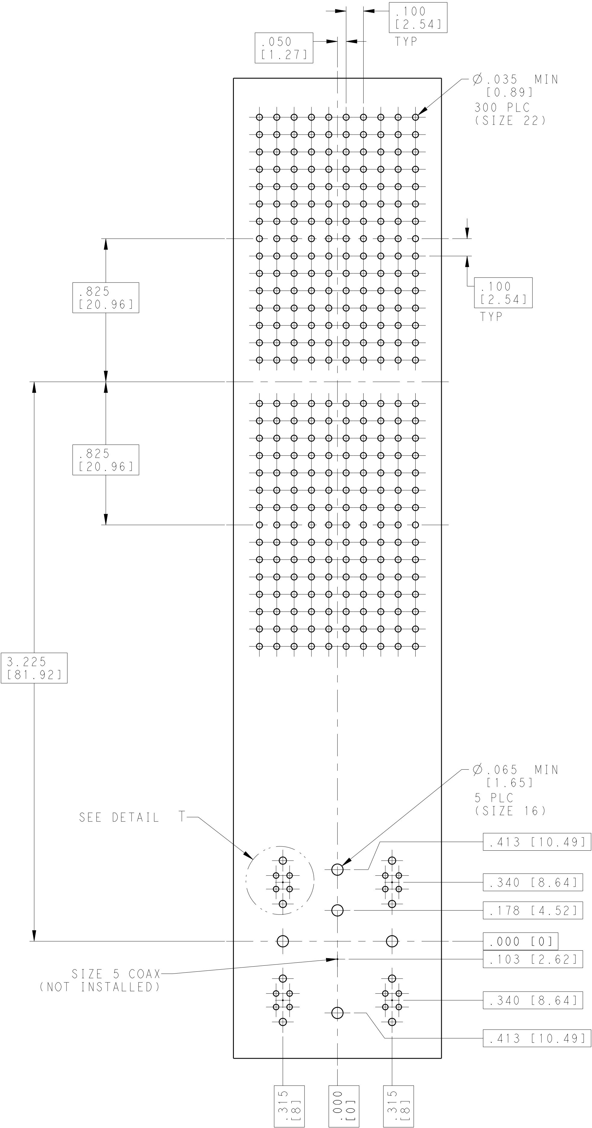
RECOMMENDED P.C. BOARD LAYOUT SCALE 3:1
