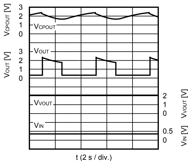
Figure 12 Steady-state Operation Waveform for Intermittently Power Supplying to Capacitor
