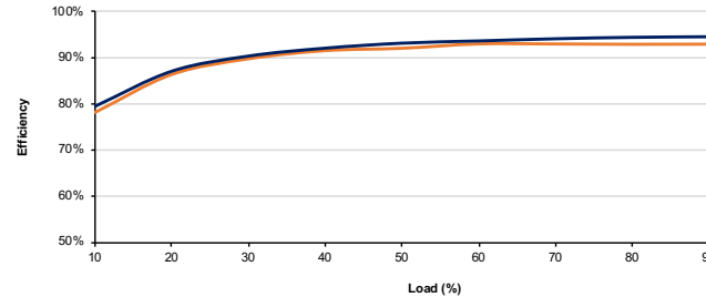
Figure 4 - ECH450PS24 (450W)
