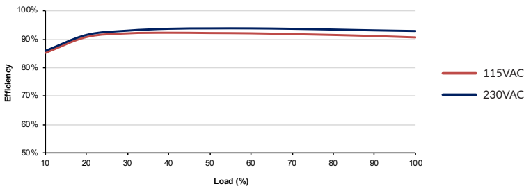
Figure 3 - ECH450PS24 (250W)
