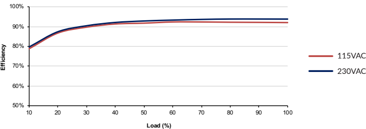
Figure 1 - ECH450PS12 (250W)
