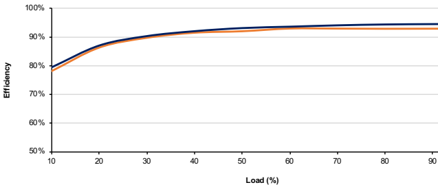
Figure 2 - ECH450PS12 (450W)
