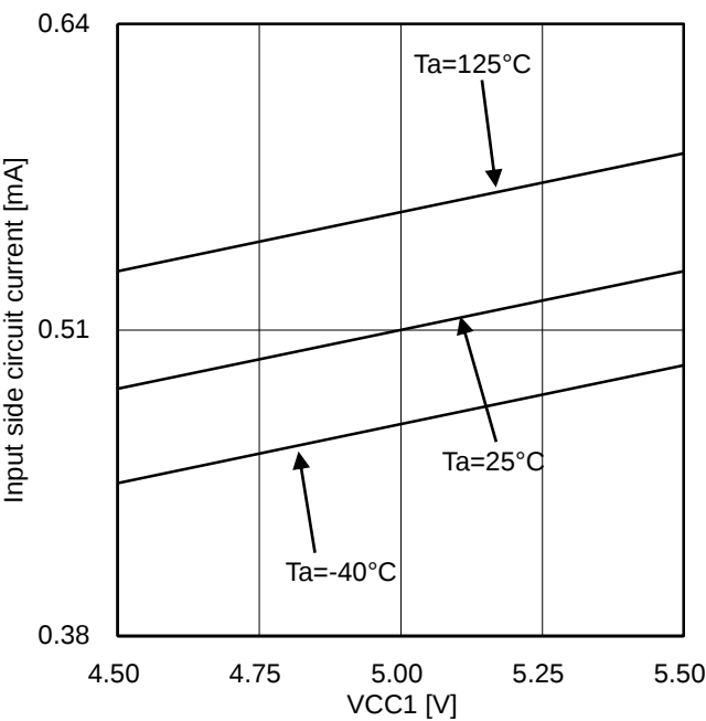
Figure 16. Input side circuit current vs. VCC1 (OUT1=L)
