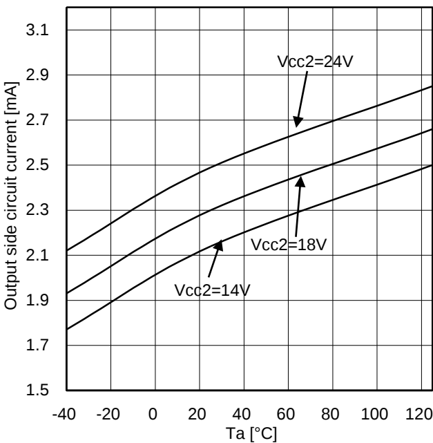
Figure 25. Output side circuit current vs. Temperature (OUT1=L)
