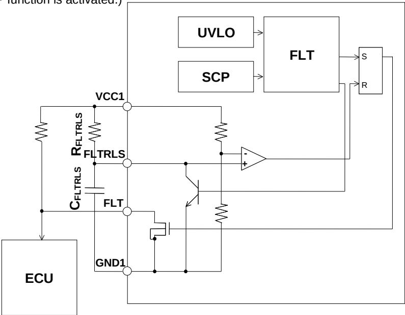
Figure 6. Fault Output Block Diagram
