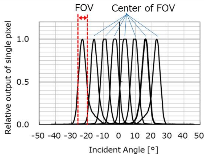
Fig. 4 FOV characteristics
