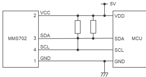
Fig. 5 Case of connecting to MCU operating at 5V
