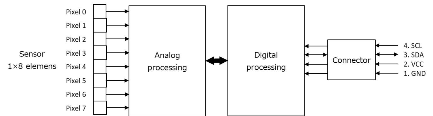
Fig. 1 Block Diagram
