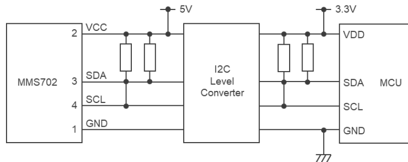
Fig. 6 Case of connecting to MCU operating at 3.3V via I2C level converter
