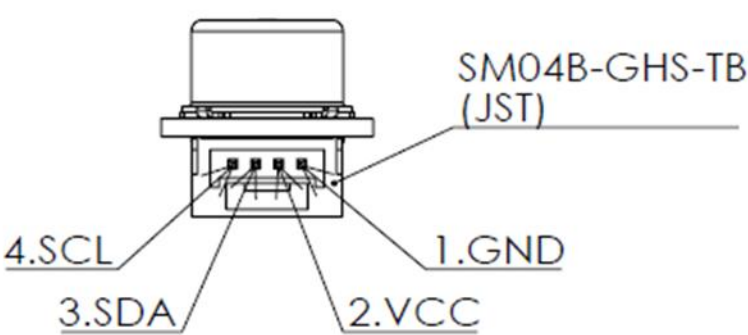
Fig. 2 Pin Configuration (Top View)
