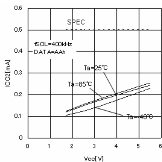
Figure 9. Consumption current at write action Icc2 (fSCL=400kHz)
