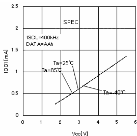
Figure 8. Consumption current at write action Icc1 (fSCL=400kHz)
