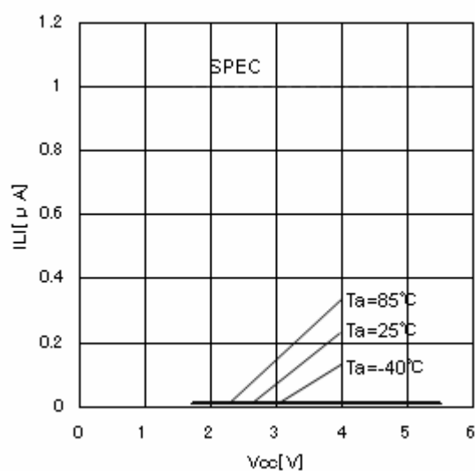
Figure 6. Input leak current ILI (A2, SCL, WP)
