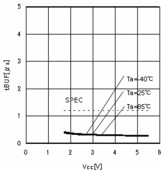
Figure 22. Bus release time before transfer start tBUF
