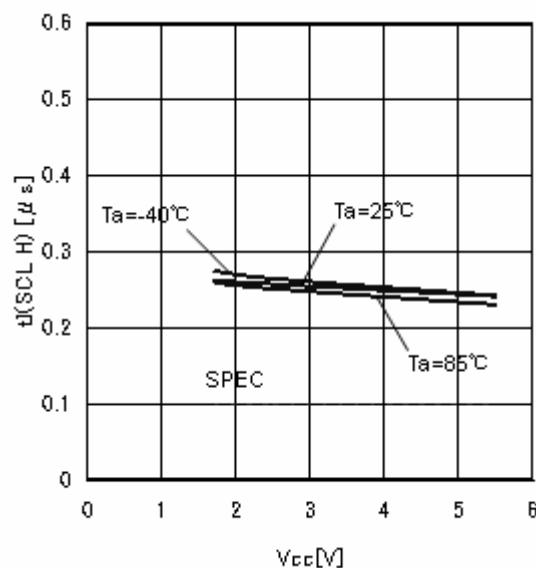
Figure 24. Noise removal time tI (SCL H)
