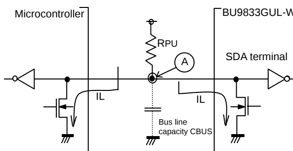
Figure 44. I/O circuit diagram
