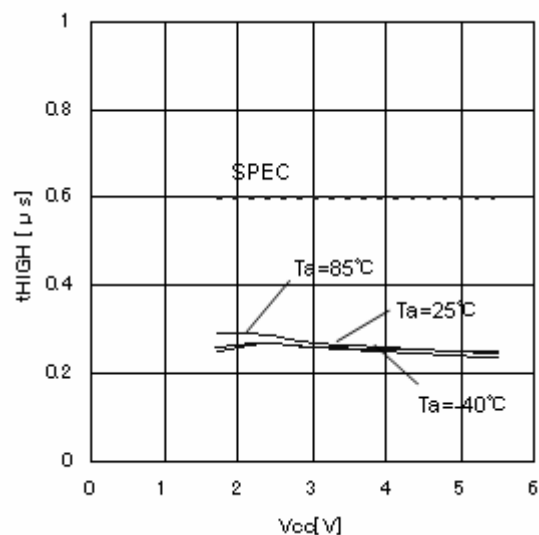
Figure 12. Data clock "H" time t_{HIGH}
