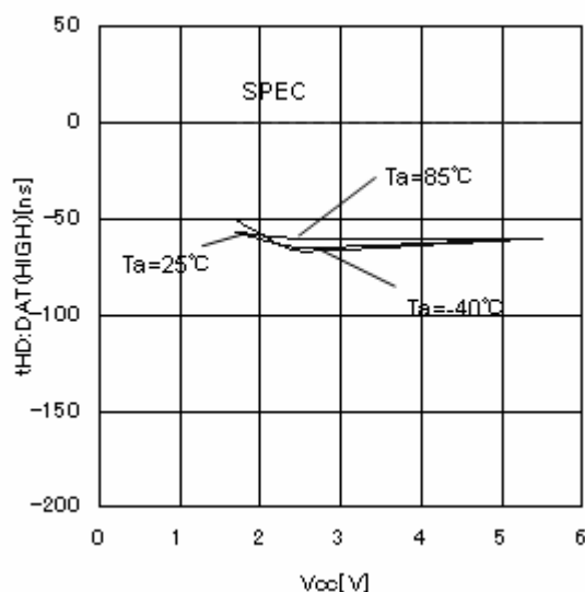
Figure 16. Input data hold time t_{HD:DAT}
