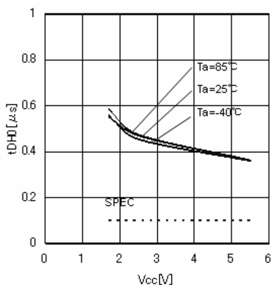
Figure 20. Output data hold time t_{DH1}
