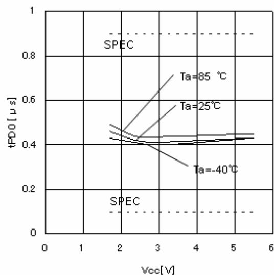
Figure 18. Output data delay time t_{PD0}
