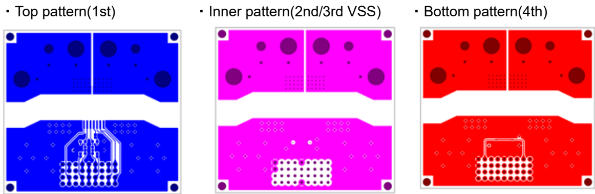
Figure 8. Board layout for measuring thermal resistance of CZ-3A03
