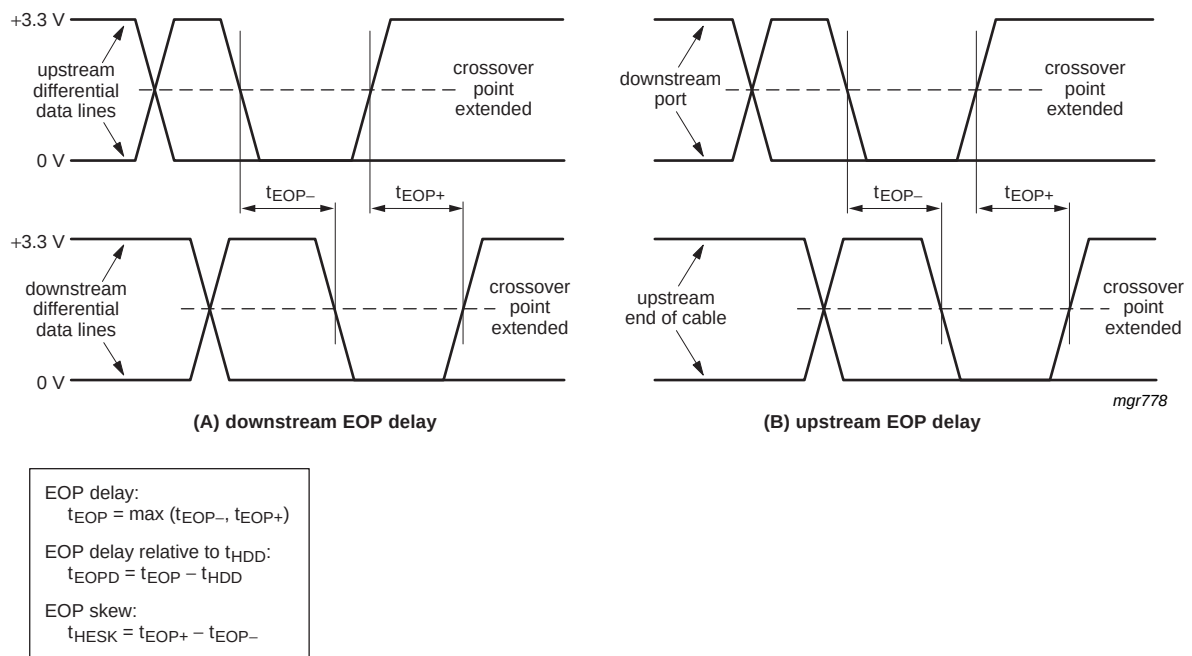
Fig 15. Hub EOP delay and EOP skew
