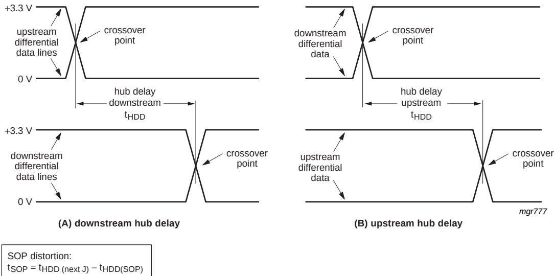
Fig 14. Hub differential data delay and SOP distortion
