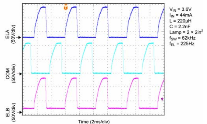
Figure 3. EL Panel Waveform – 2 \times 2 in^2
