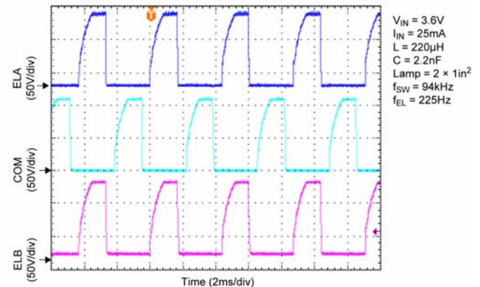
Figure 2. EL Panel Waveform – 2 \times 1 in^2
