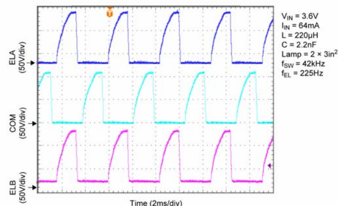
Figure 4. EL Panel Waveform – 2 \times 3 in^2
