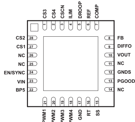
RHD PACKAGE (BOTTOM VIEW)
