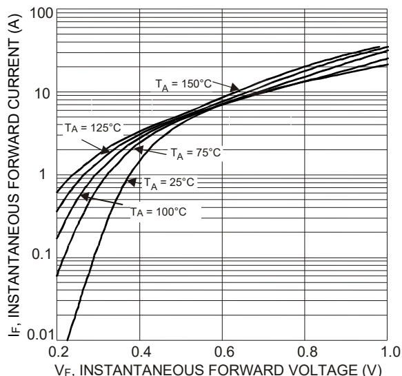
Fig. 1 Typical Forward Characteristics - B320AQ thru B340AQ
