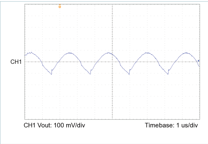
Figure 17 — Output voltage ripple, V_{IN} = 28\text{ V} , V_{OUT} = 5.0\text{ V} , C_{OUT\_EXT} = 1000\text{ }\mu\text{F} , R_{LOAD} = 0.139\text{ }\Omega
