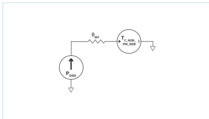
Figure 19 – Single-sided cooling VIA thermal model
