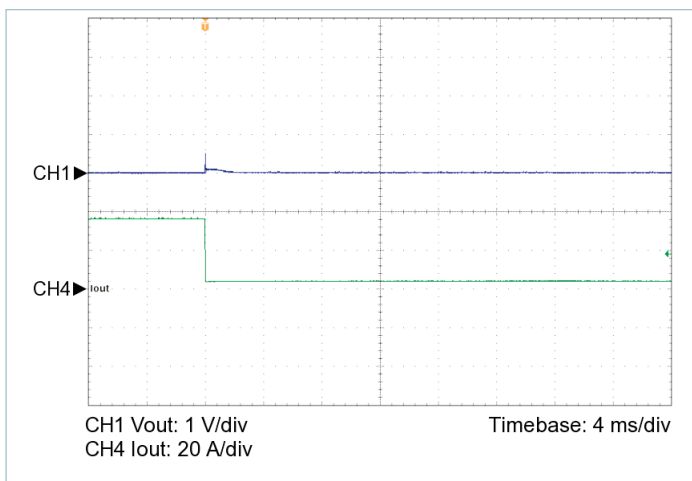
Figure 5 — 100% to 10% load transient response, V_{IN} = 28\text{ V} , nominal trim, C_{OUT\_EXT} = 1000\text{ }\mu\text{F}
