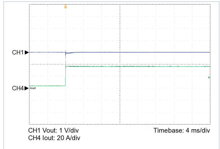
Figure 6 — 10% to 100% load transient response, V_{IN} = 28\text{ V} , nominal trim, C_{OUT\_EXT} = 1000\text{ }\mu\text{F}
