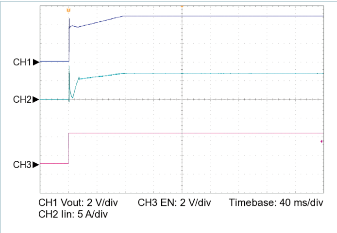
Figure 15 — Startup from EN, V_{IN} = 28\text{ V} , C_{OUT\_EXT} = 20000\text{ }\mu\text{F} , R_{LOAD} = 0.139\text{ }\Omega
