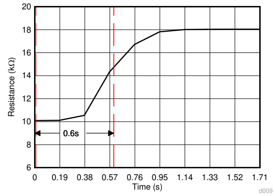
Figure 6-8. Thermal Response Time (DEC package)
