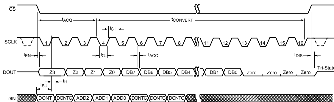
Figure 4. ADC082S051 Serial Timing Diagram
