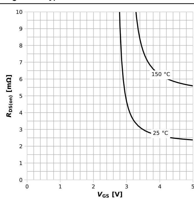
Diagram 10: Typ. Drain-source on-state resistance
