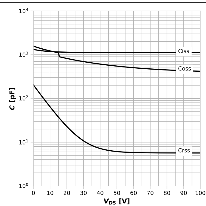
Diagram 13: Typ. capacitances
