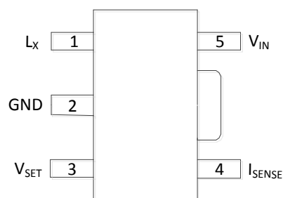
SOT89-5
