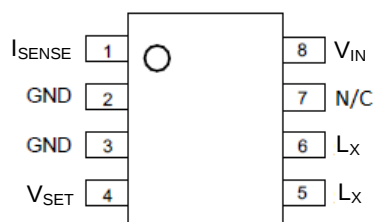
MSOP-8EP
