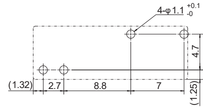
PC board mounting hole layout (BOTTOM VIEW)
