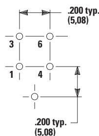
PC Mounting
