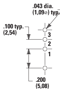
PC Mounting
