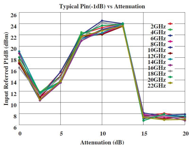
Typical Pin (1dB) vs Attenuation
