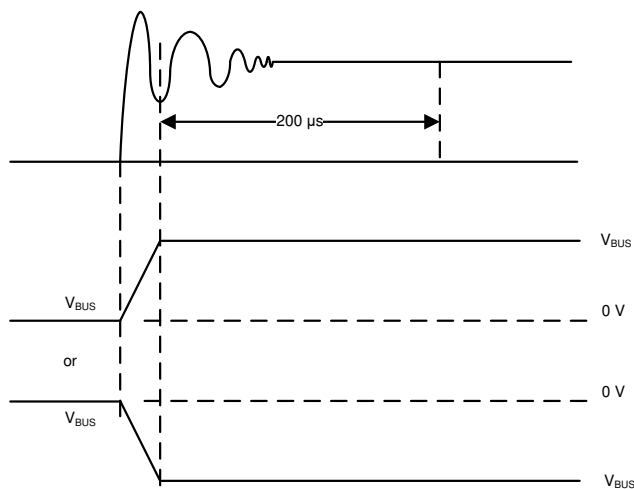
Figure 9-8. Driver Short-Circuit Current Test and Measurement
