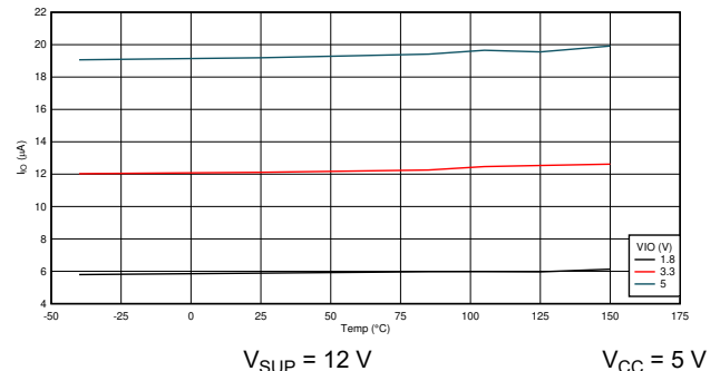
Figure 8-6. Normal Mode: I_{IO} vs Temperature Dominant
