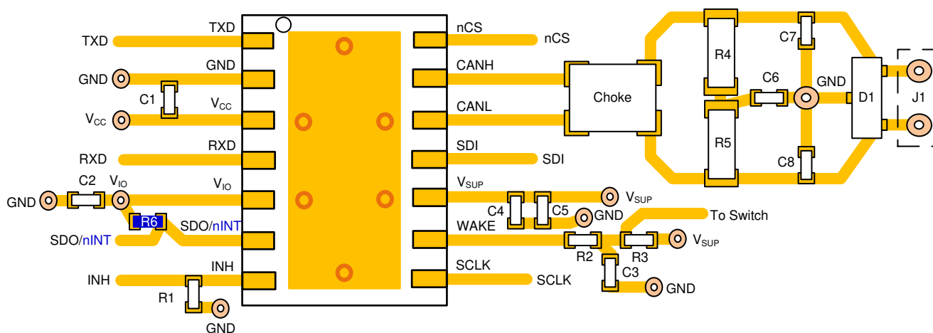
Figure 13-1. Example Layout
