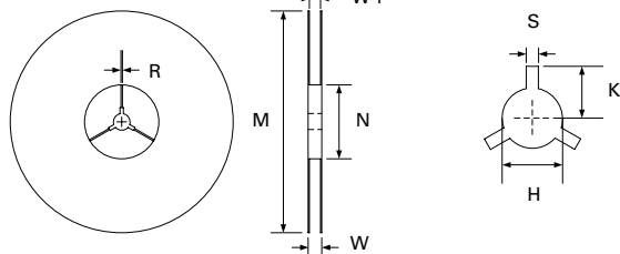
Reel Size 7 Inch
