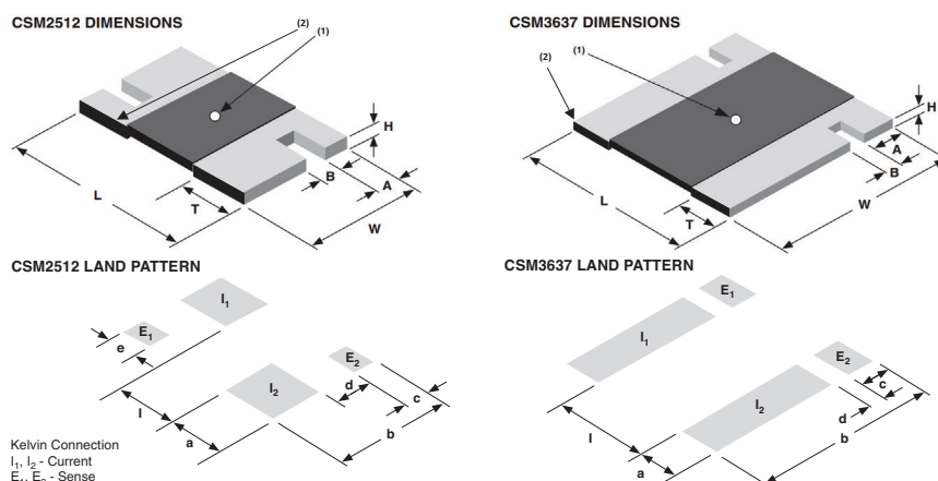
Figure 2 – Dimensions and Imprinting in inches (millimeters)
