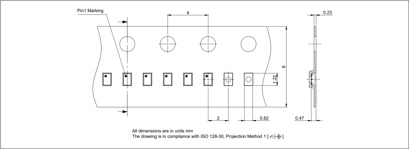
Figure 6: PG-TSnp-6-10 Carrier Tape
