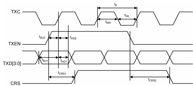
Figure 10. MII Transmit Timing (10Base-T)
