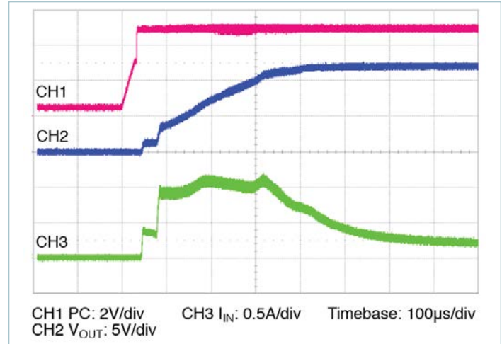
Figure 14 — Start up from application of PC; V_{IN} pre-applied C_{OUT} = 1000\mu F
