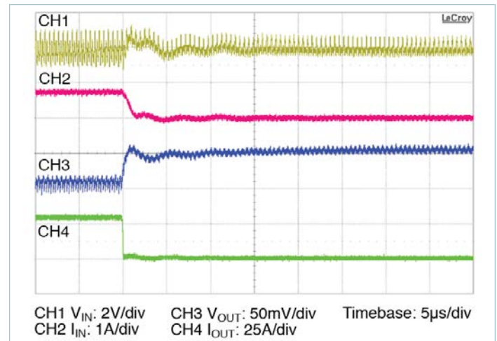
Figure 16 — 27.3A – 0A transient response: C_{IN} = 1\mu F , I_{IN} measured prior to C_{IN} , no external C_{OUT}
