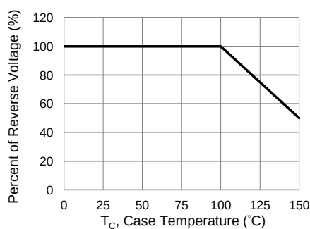
Fig.5 Operating Temperature Derating Curve
