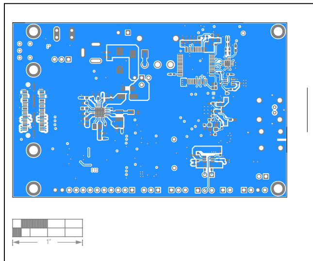
MAX96717 EV Kit—Bottom
