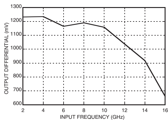
Output Differential vs. Frequency [3]
