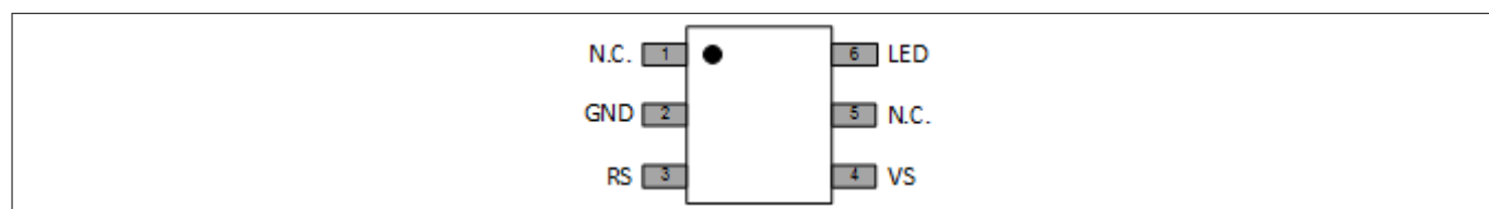
Figure 2 Pinout BCR430U
