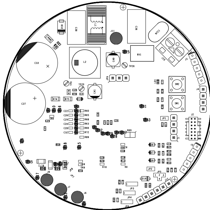
Figure 5. EVLPWD-FAN-PUMP layout - component placement (bottom view)
