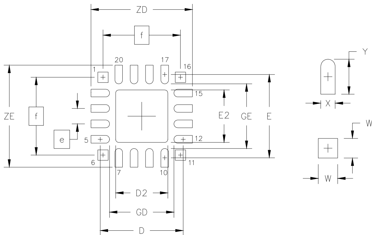
Figure 7. PCB Land Pattern
