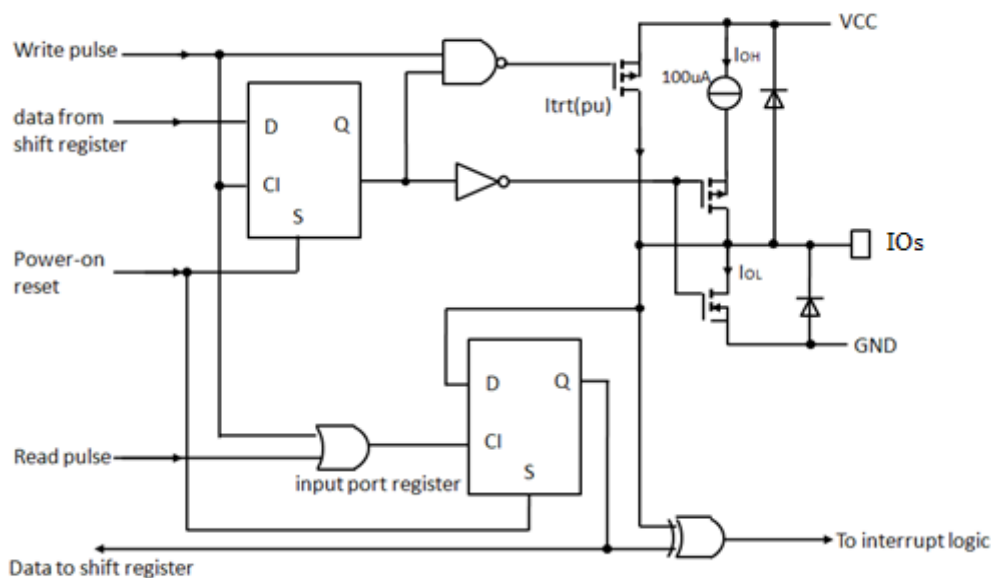
Fig 3. Simplified schematic diagram of IOX_0 to IOX_7
