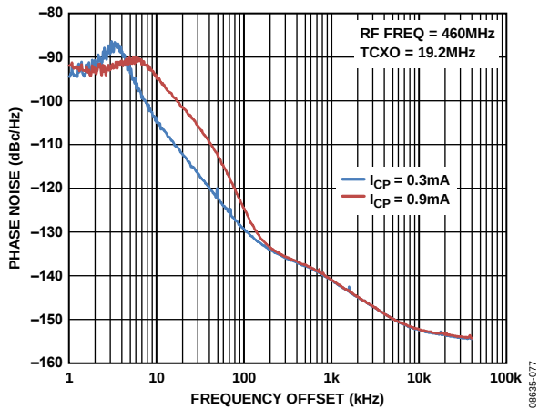
Figure 11. Phase Noise Response at 460 MHz, V_{DD} = 3\text{ V}
