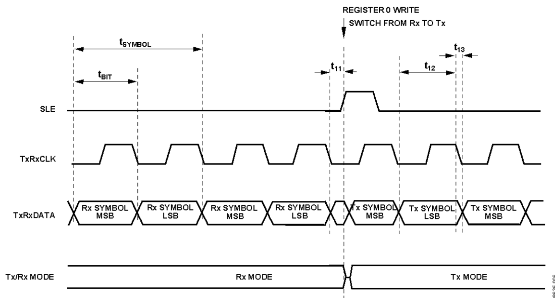
Figure 6. Receive-to-Transmit Timing Diagram in 4FSK Mode
