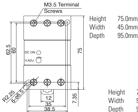
PS5R-Q (75W)
