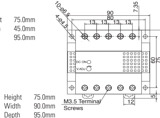
PS5R-F (120W)
