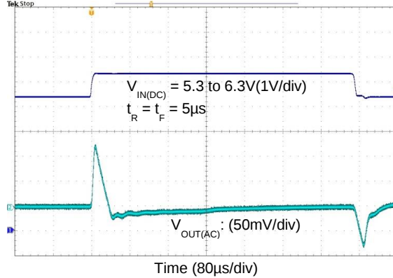
Line-Transient Response
