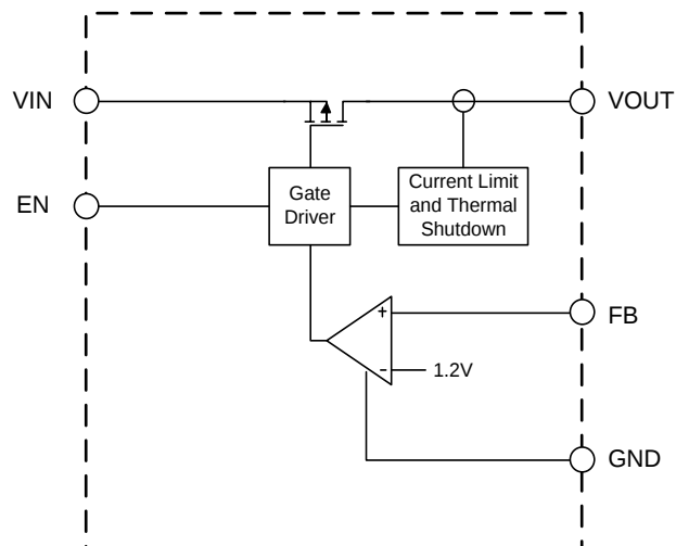
AP7583Q Adjustable Version
