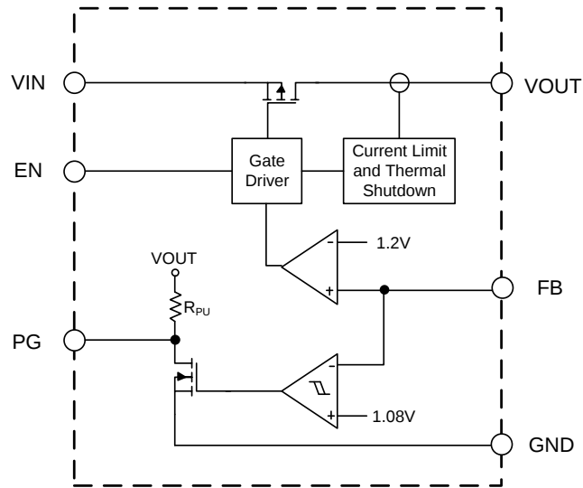
AP7583AQ Adjustable Version
