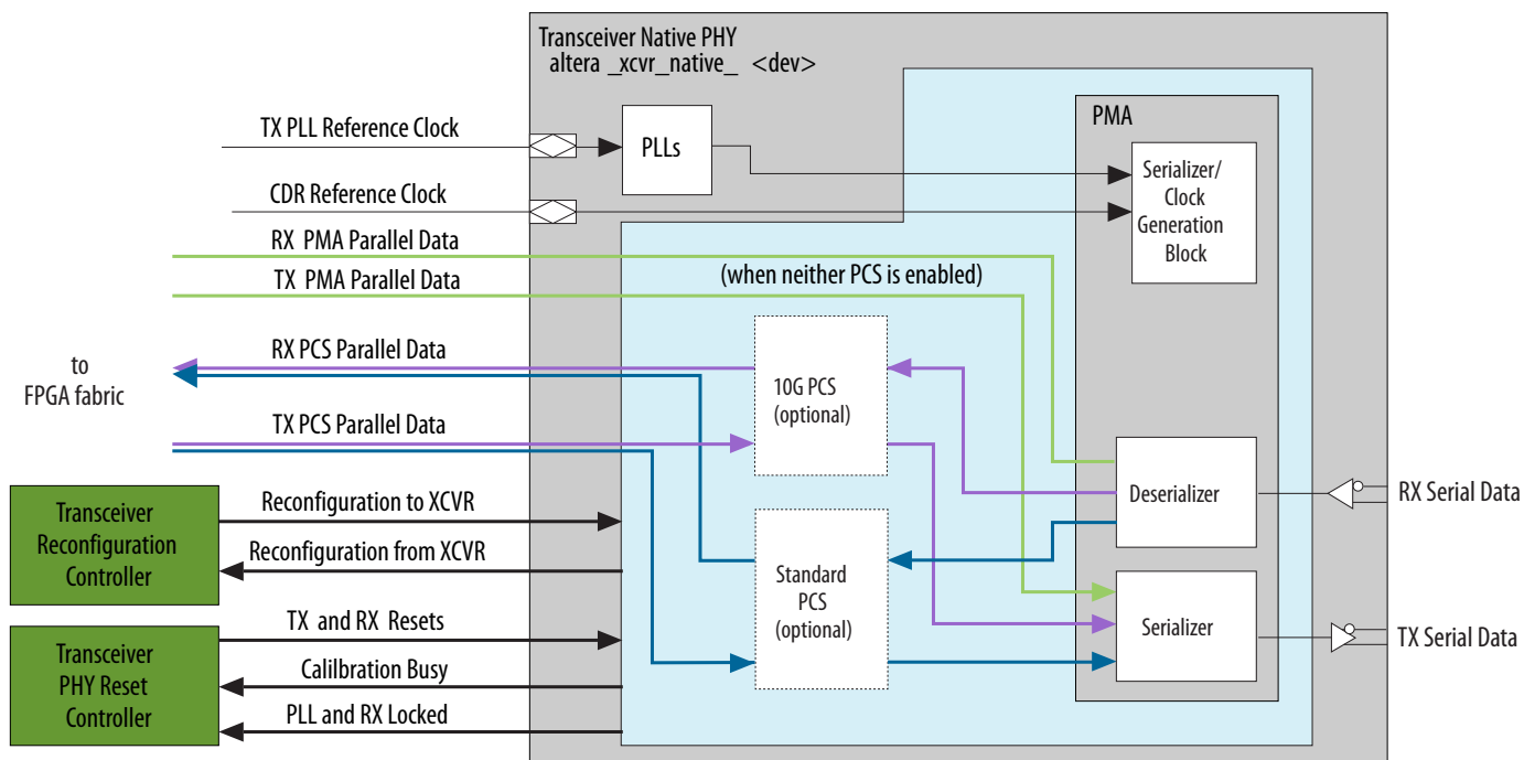
Figure 13-1: Stratix V Native Transceiver PHY IP Core
