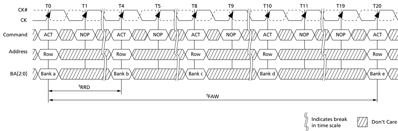
Figure 64: Example: t_{FAW}
