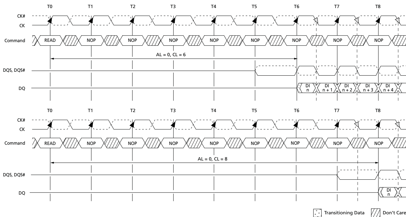
Figure 51: READ Latency
