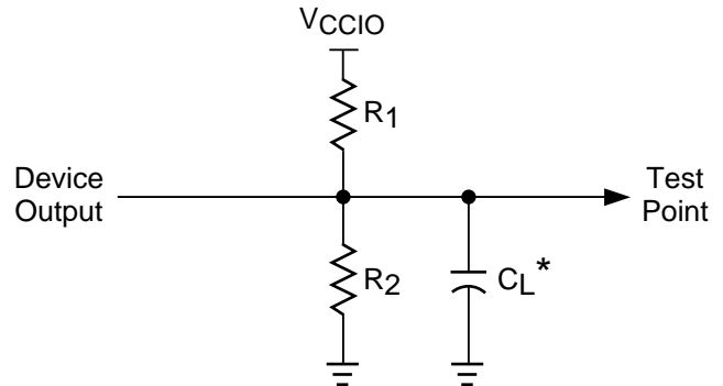
Figure 8. Test Load
