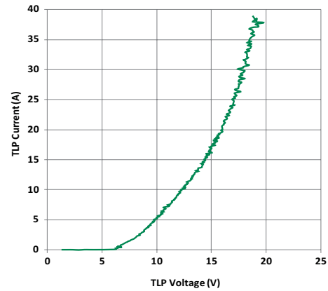
Transmission Line Pulsing (TLP) Plot (Pin 1 to Pin2)
