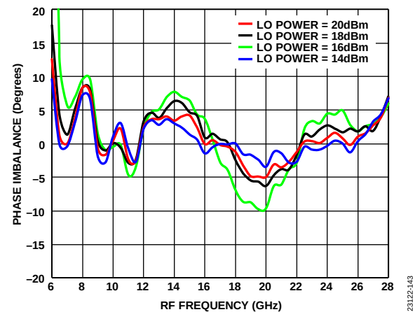
Figure 143. Phase Imbalance vs. RF Frequency at Various LO Drives, IF = 100 MHz, T_A = 25^\circ\text{C}
