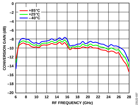
Figure 37. Conversion Gain vs. RF Frequency at Various Temperatures, LO Drive = 18 dBm
