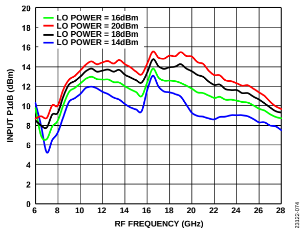
Figure 74. Input P1dB vs. RF Frequency at Various LO Drives, T_A = 25^\circ\text{C}
