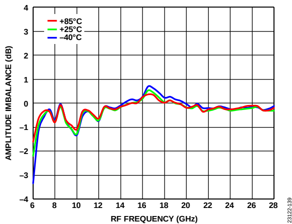
Figure 139. Amplitude Imbalance vs. RF Frequency at Various Temperatures, LO Drive = 18 dBm, IF = 100 MHz
