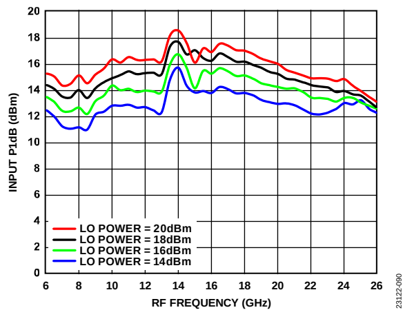
Figure 90. Input P1dB vs. RF Frequency at Various LO Drives, T_A = 25^\circ\text{C}
