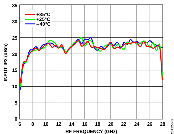
Figure 39. Input IP3 vs. RF Frequency at Various Temperatures, LO Drive = 18 dBm
