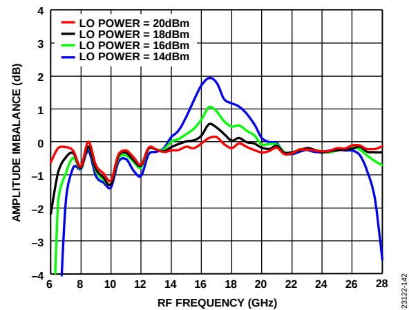
Figure 142. Amplitude Imbalance vs. RF Frequency at Various LO Drives, IF = 100 MHz, T_A = 25^\circ\text{C}
