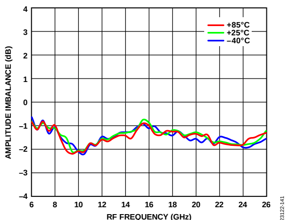
Figure 141. Amplitude Imbalance vs. RF Frequency at Various Temperatures, LO Drive = 18 dBm, IF = 2500 MHz
