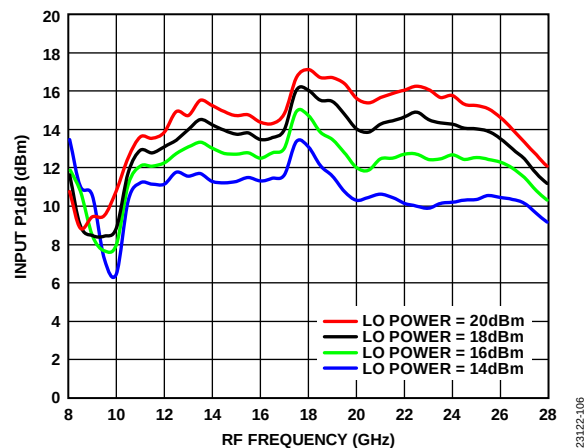
Figure 106. Input P1dB vs. RF Frequency at Various LO Drives, TA = 25°C
