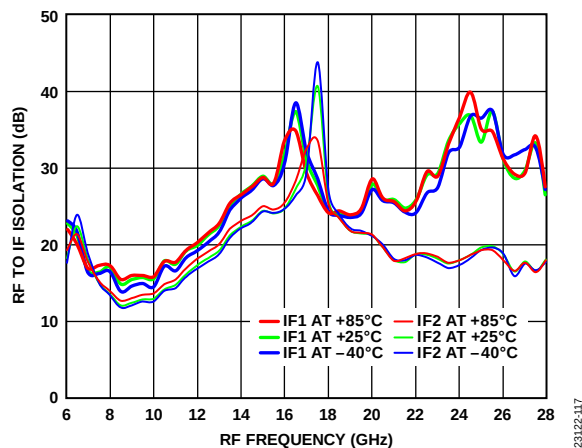
Figure 117. RF to IF Isolation vs. RF Frequency at Various IFx Temperatures, IF = 100 MHz, LO Drive = 18 dBm
