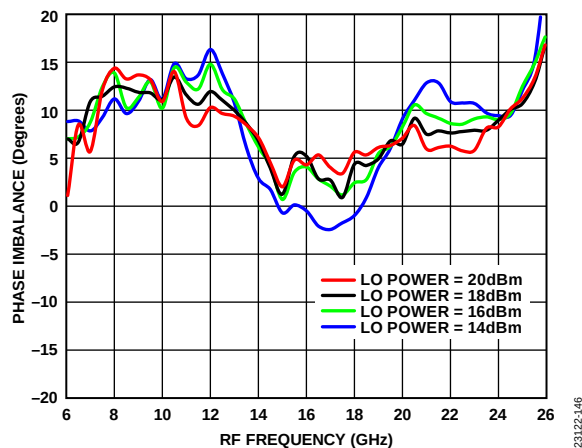
Figure 146. Phase Imbalance vs. RF Frequency at Various LO Drives, IF = 2500 MHz, T_A = 25^\circ\text{C}
