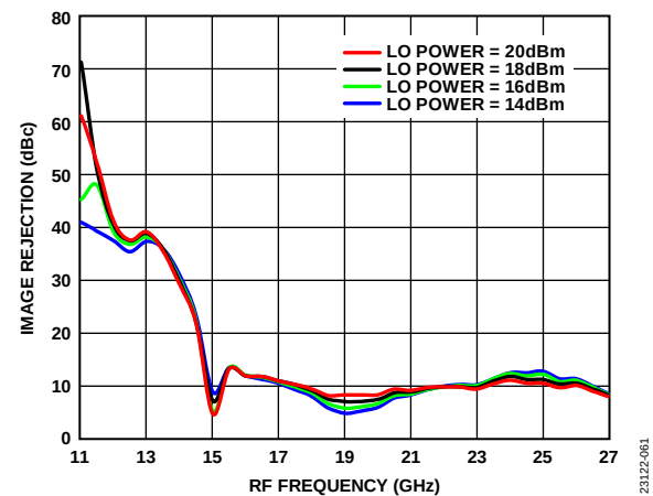
Figure 61. Image Rejection vs. RF Frequency at Various LO Drives, T_A = 25^\circ\text{C}
