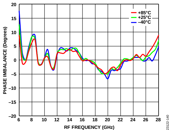
Figure 140. Phase Imbalance vs. RF Frequency at Various Temperatures, LO Drive = 18 dBm, IF = 100 MHz
