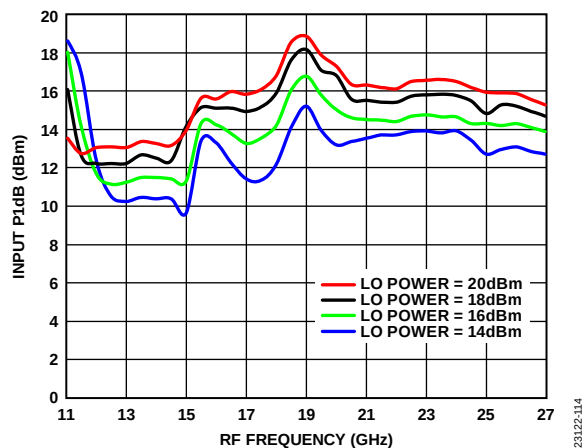
Figure 114. Input P1dB vs. RF Frequency at Various LO Drives, T_A = 25^\circ\text{C}
