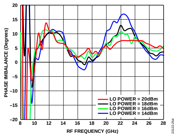
Figure 154. Phase Imbalance vs. RF Frequency at Various LO Drives, IF = 2500 MHz, T_A = 25^\circ\text{C}
