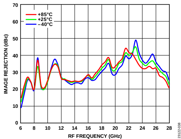
Figure 38. Image Rejection vs. RF Frequency at Various Temperatures, LO Drive = 18 dBm
