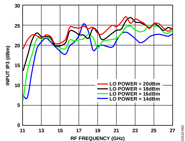
Figure 62. Input IP3 vs. RF Frequency at Various LO Drives, T_A = 25^\circ\text{C}
