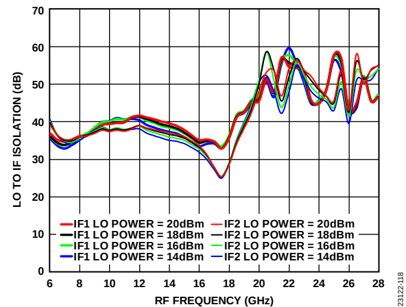
Figure 118. LO to IF Isolation vs. RF Frequency at Various IFx LO Drives, IF = 100 MHz, T A = 25°C
