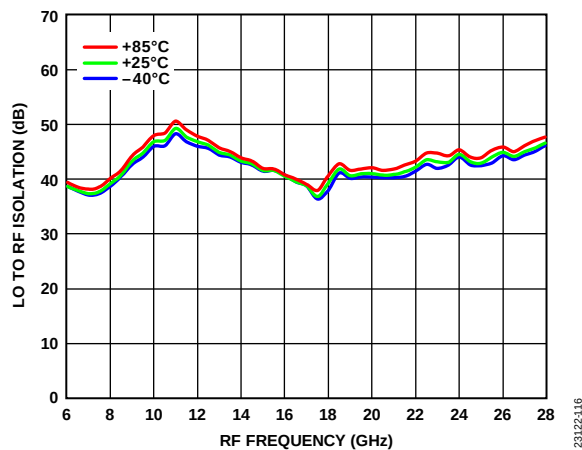
Figure 116. LO to RF Isolation vs. RF Frequency at Various Temperatures, IF = 100 MHz, LO Drive = 18 dBm
