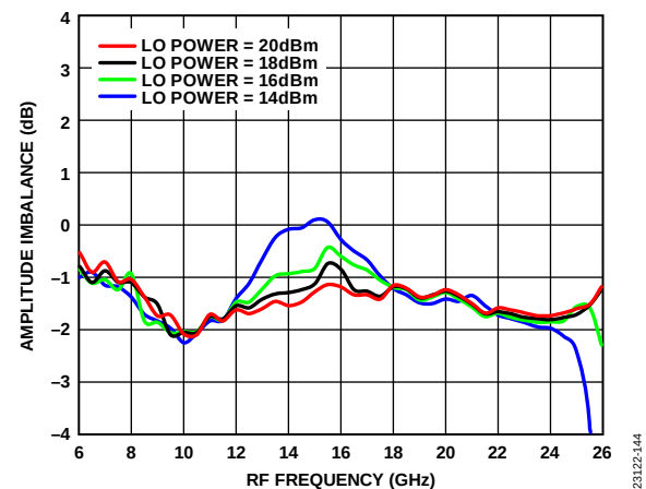
Figure 144. Amplitude Imbalance vs. RF Frequency at Various LO Drives, IF = 2500 MHz, T_A = 25^\circ\text{C}
