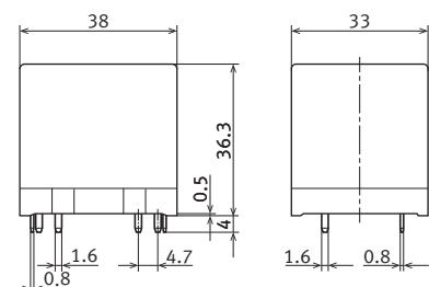
External dimensions
