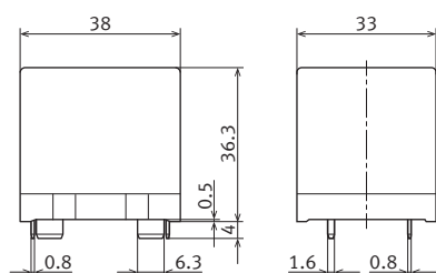
External dimensions
