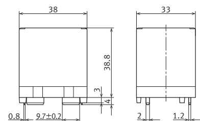
External dimensions
