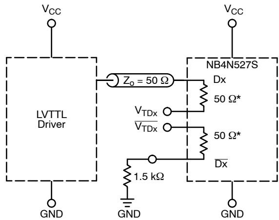
Figure 12. LVTTTL Interface
