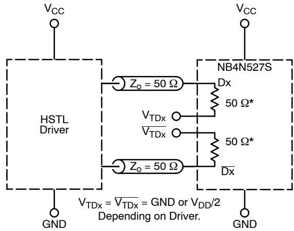
Figure 10. HSTL Interface
