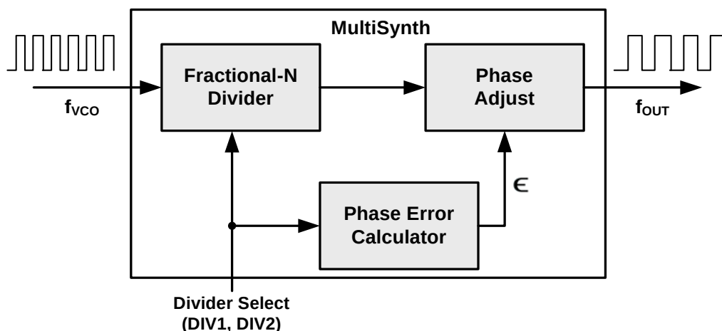
Figure 3. Silicon Labs' MultiSynth Technology
