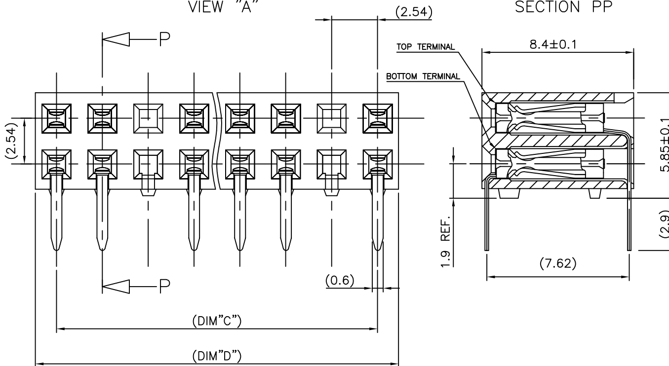
VIEW "A"
